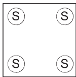
PATTERN A Corner mount 4 swivel casters
