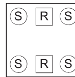
PATTERN E Full mount 2 rigid/4 swivel casters (Where added strength is needed)
